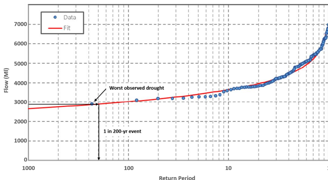
Figure 21 Example of Extreme Value Analysis to estimate drought return periods
