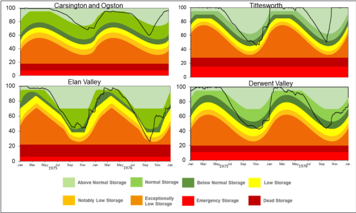
Figure 23 Reservoir Storage during Design Drought
