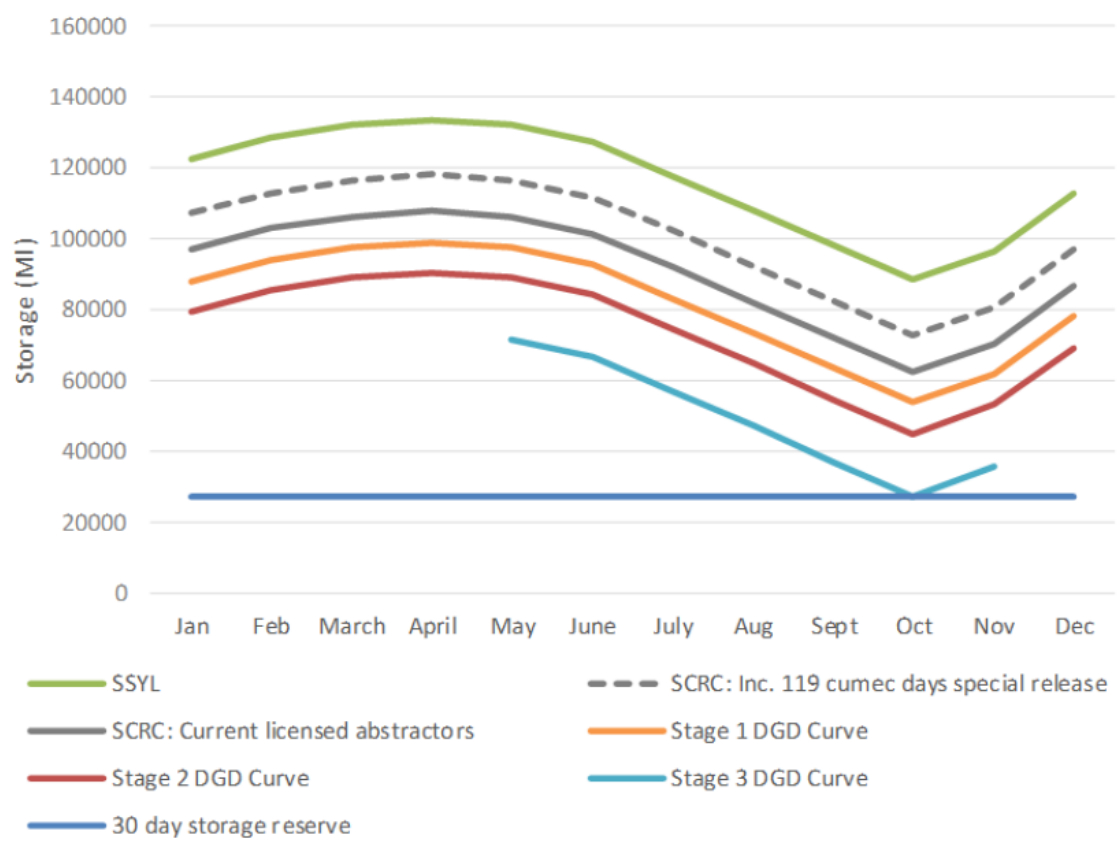
Figure 17 - Dee Storage System conservation rule curve and drought management curves
