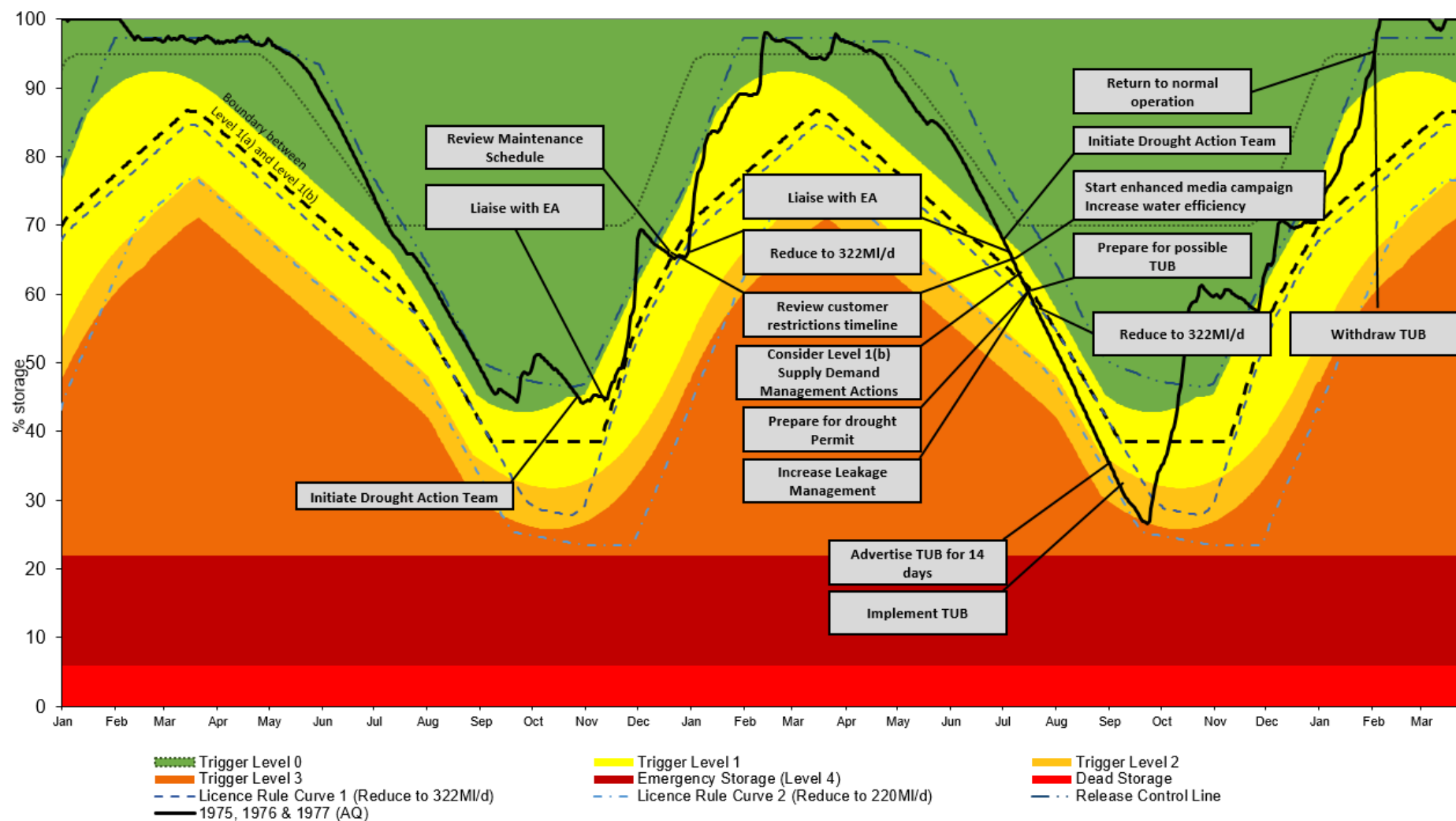
Figure 14 Elan Valley example dry year 1975-1976 drawdown and the annotated demand-side and supply-side actions
